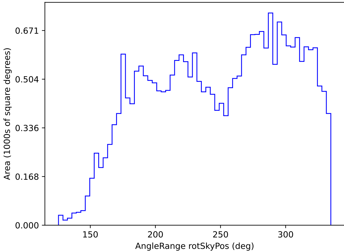
noroll_mjdp365_v3.4_10yrs All sky g band: AngleRange rotSkyPos
