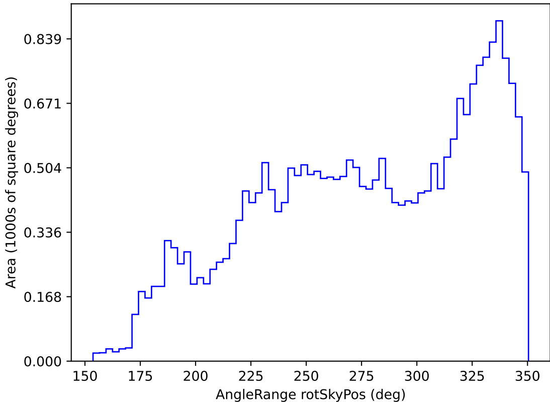
noroll_mjdp365_v3.4_10yrs All sky all bands: AngleRange rotSkyPos
