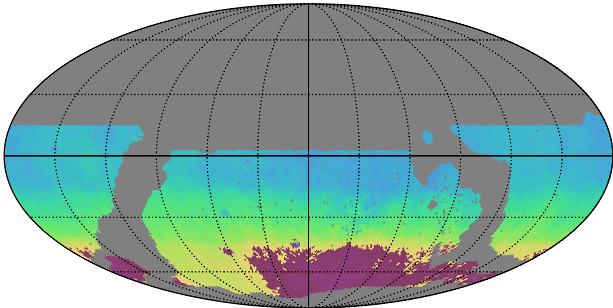
noroll_mjdp365_v3.4_10yrs WFD y band: AngleMean rotSkyPos
