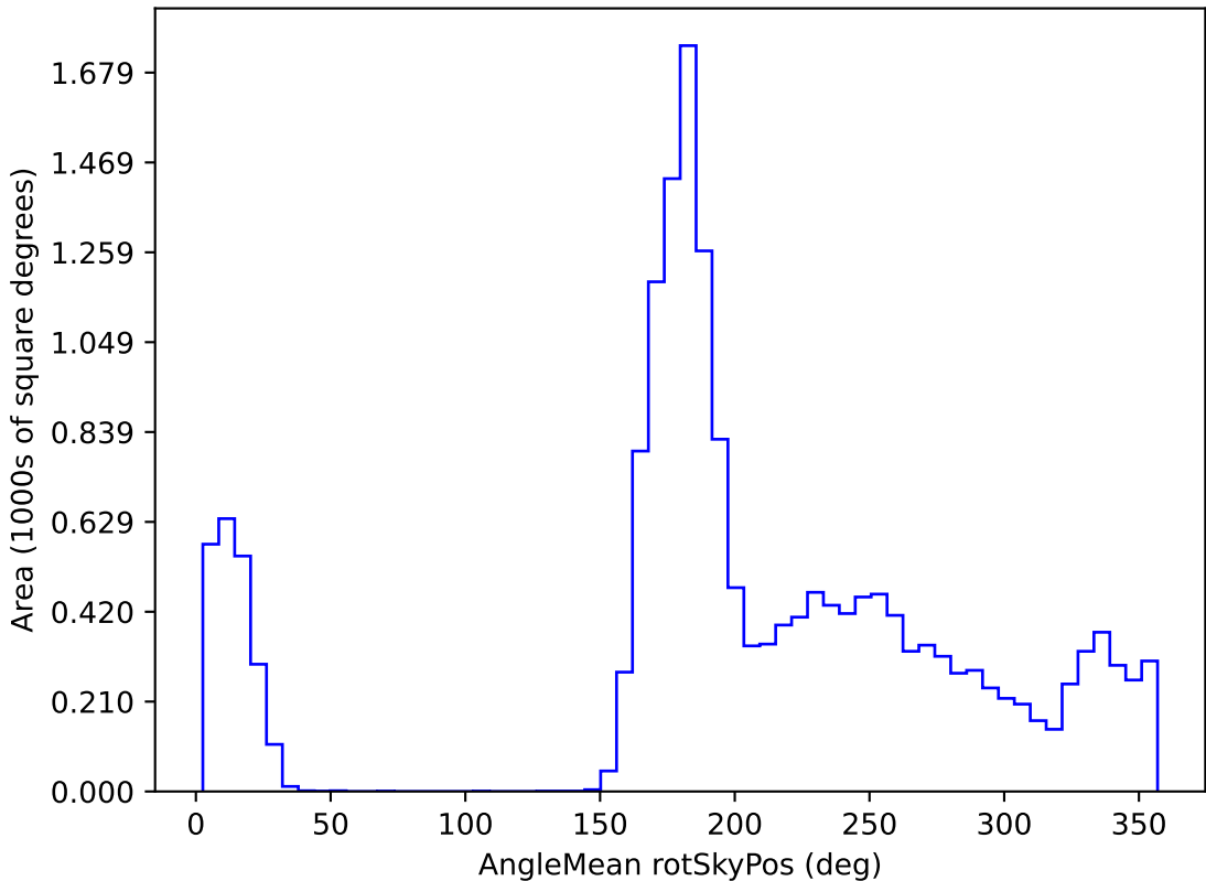
noroll_mjdp365_v3.4_10yrs WFD y band: AngleMean rotSkyPos
