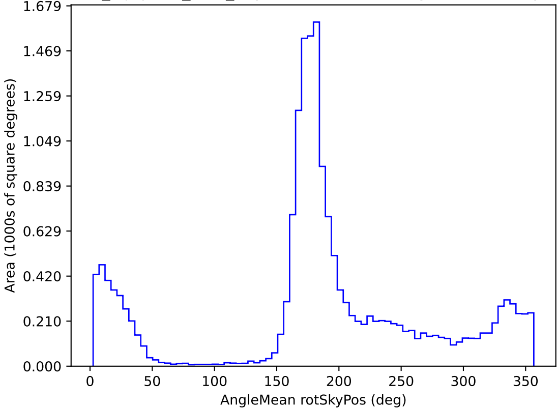
noroll_mjdp365_v3.4_10yrs WFD u band: AngleMean rotSkyPos
