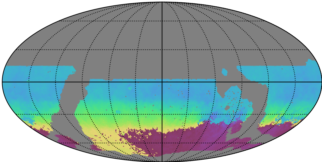
noroll_mjdp365_v3.4_10yrs WFD r band: AngleMean rotSkyPos
