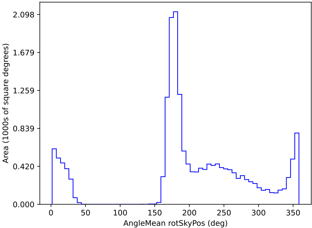
noroll_mjdp365_v3.4_10yrs WFD i band: AngleMean rotSkyPos
