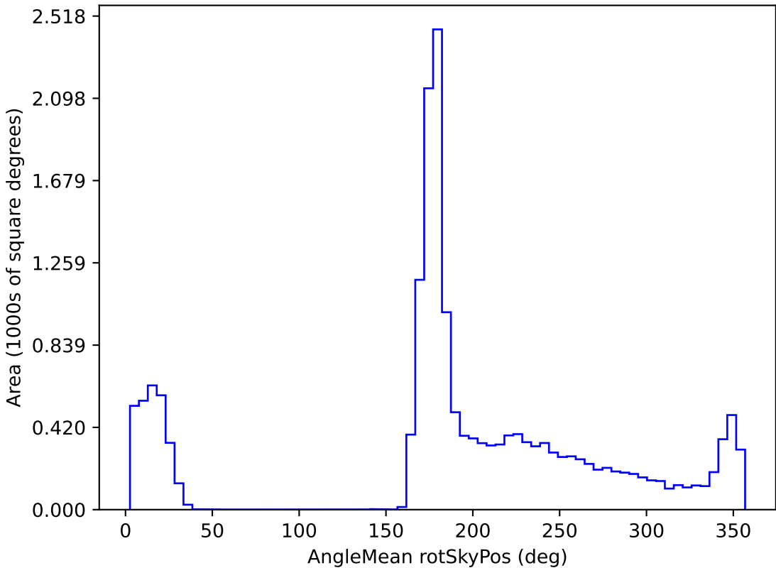
noroll_mjdp365_v3.4_10yrs WFD all bands: AngleMean rotSkyPos
