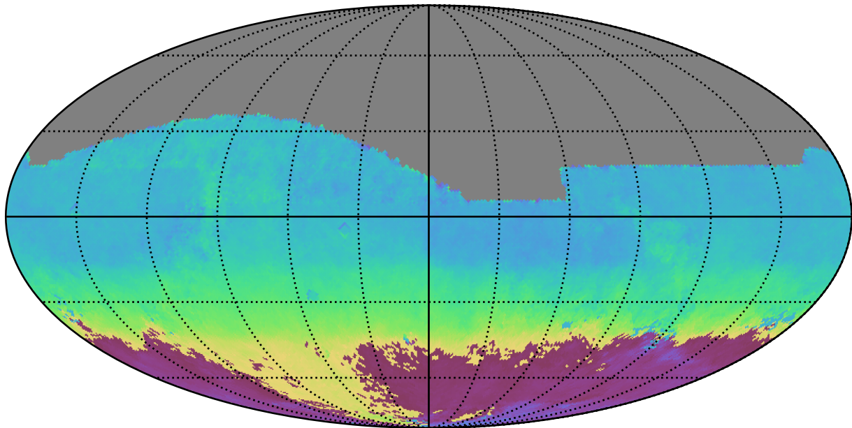
noroll_mjdp365_v3.4_10yrs All sky z band: AngleMean rotSkyPos
