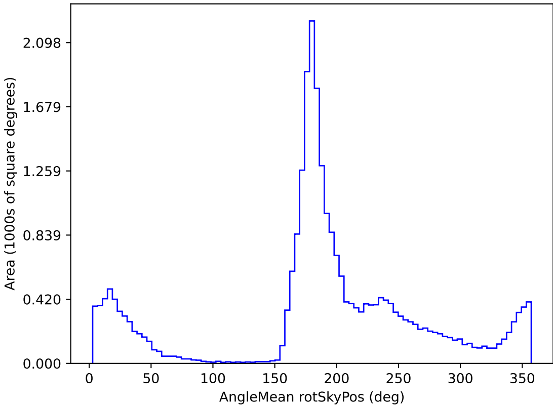
noroll_mjdp365_v3.4_10yrs All sky z band: AngleMean rotSkyPos
