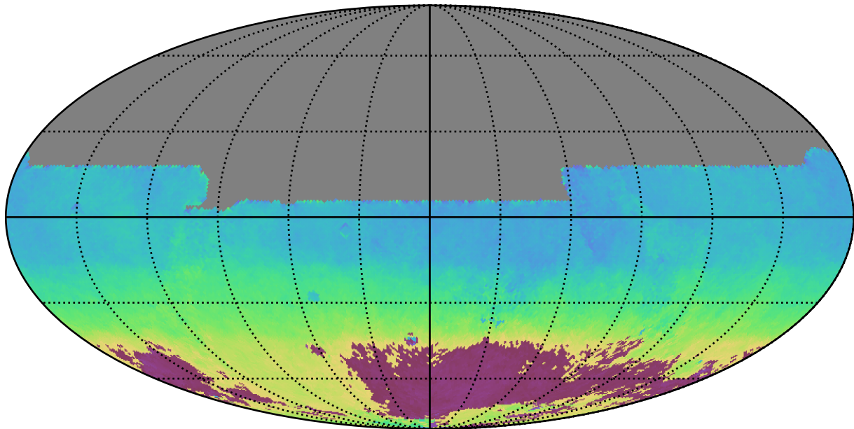
noroll_mjdp365_v3.4_10yrs All sky y band: AngleMean rotSkyPos
