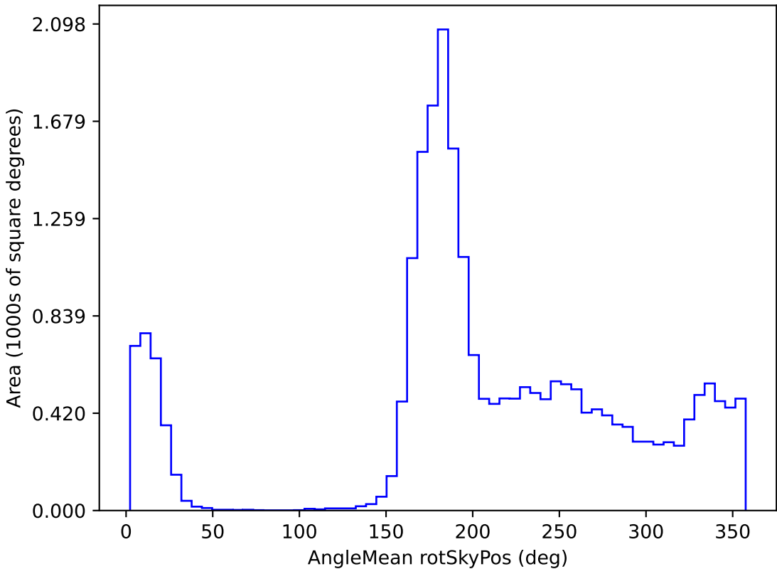
noroll_mjdp365_v3.4_10yrs All sky y band: AngleMean rotSkyPos
