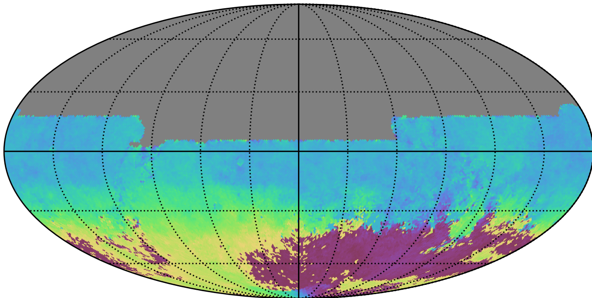
noroll_mjdp365_v3.4_10yrs All sky u band: AngleMean rotSkyPos
