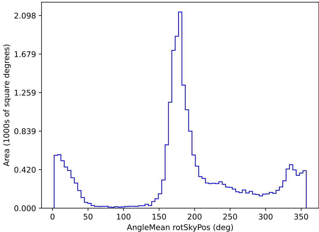
noroll_mjdp365_v3.4_10yrs All sky u band: AngleMean rotSkyPos
