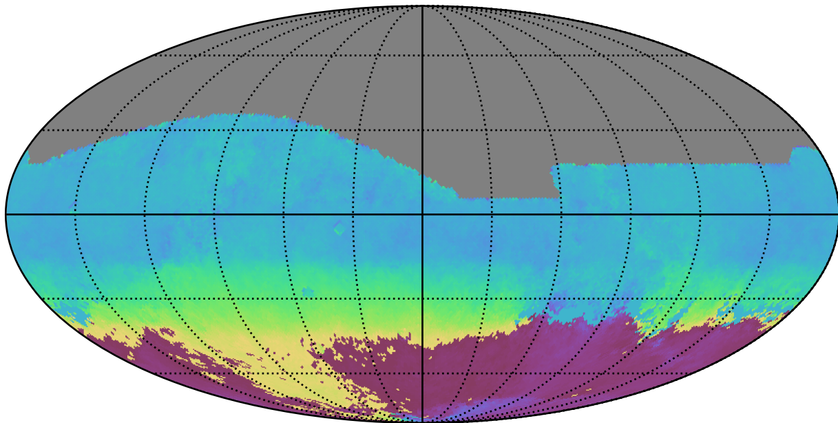
noroll_mjdp365_v3.4_10yrs All sky r band: AngleMean rotSkyPos
