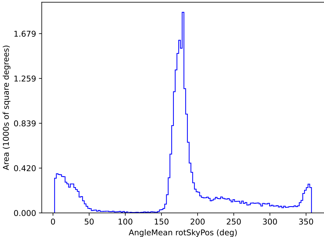
noroll_mjdp365_v3.4_10yrs All sky r band: AngleMean rotSkyPos
