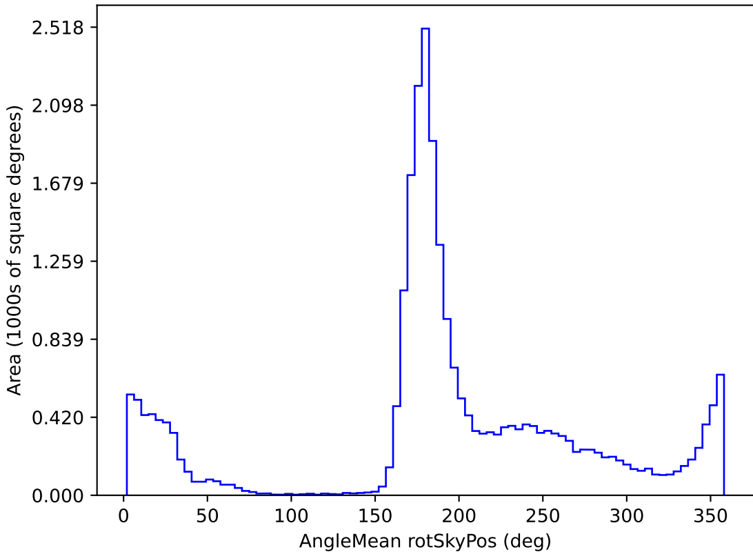
noroll_mjdp365_v3.4_10yrs All sky i band: AngleMean rotSkyPos
