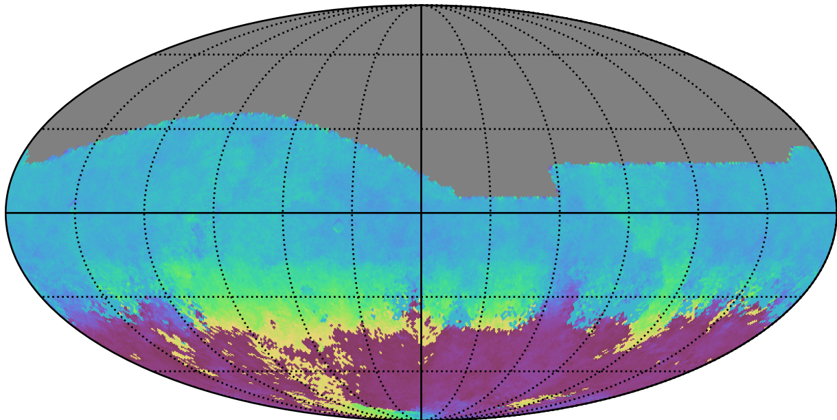
noroll_mjdp365_v3.4_10yrs All sky g band: AngleMean rotSkyPos
