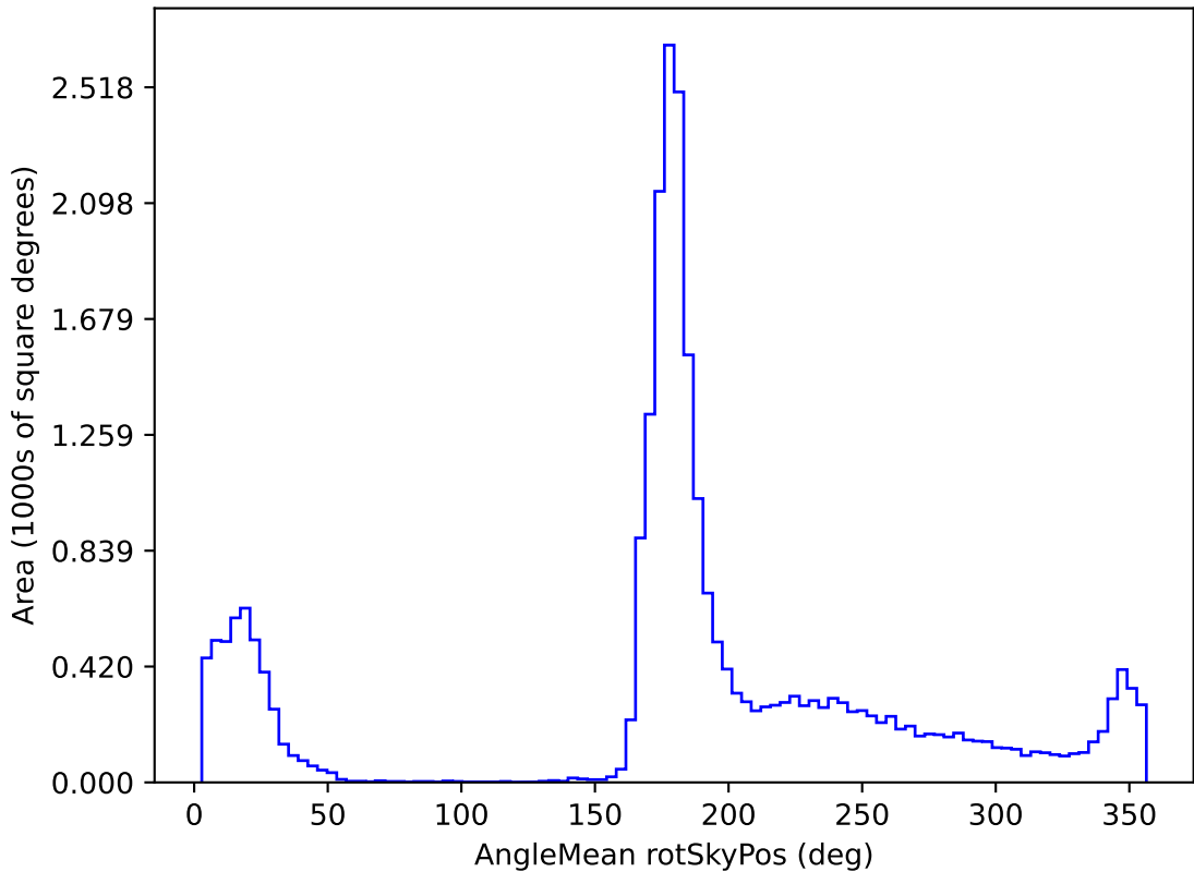
noroll_mjdp365_v3.4_10yrs All sky all bands: AngleMean rotSkyPos
