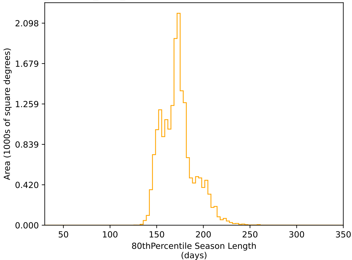
noroll_mjdp365_v3.4_10yrs WFD r band: 80thPercentile Season Length
