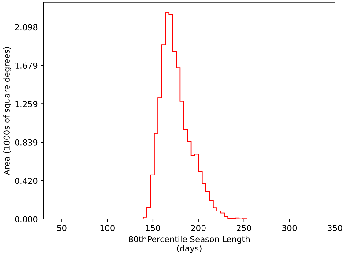
noroll_mjdp365_v3.4_10yrs WFD i band: 80thPercentile Season Length
