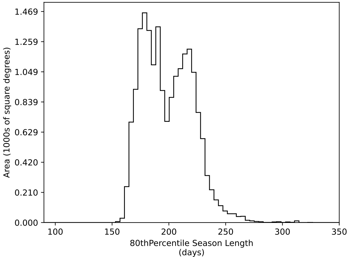
noroll_mjdp365_v3.4_10yrs WFD all bands: 80thPercentile Season Length
