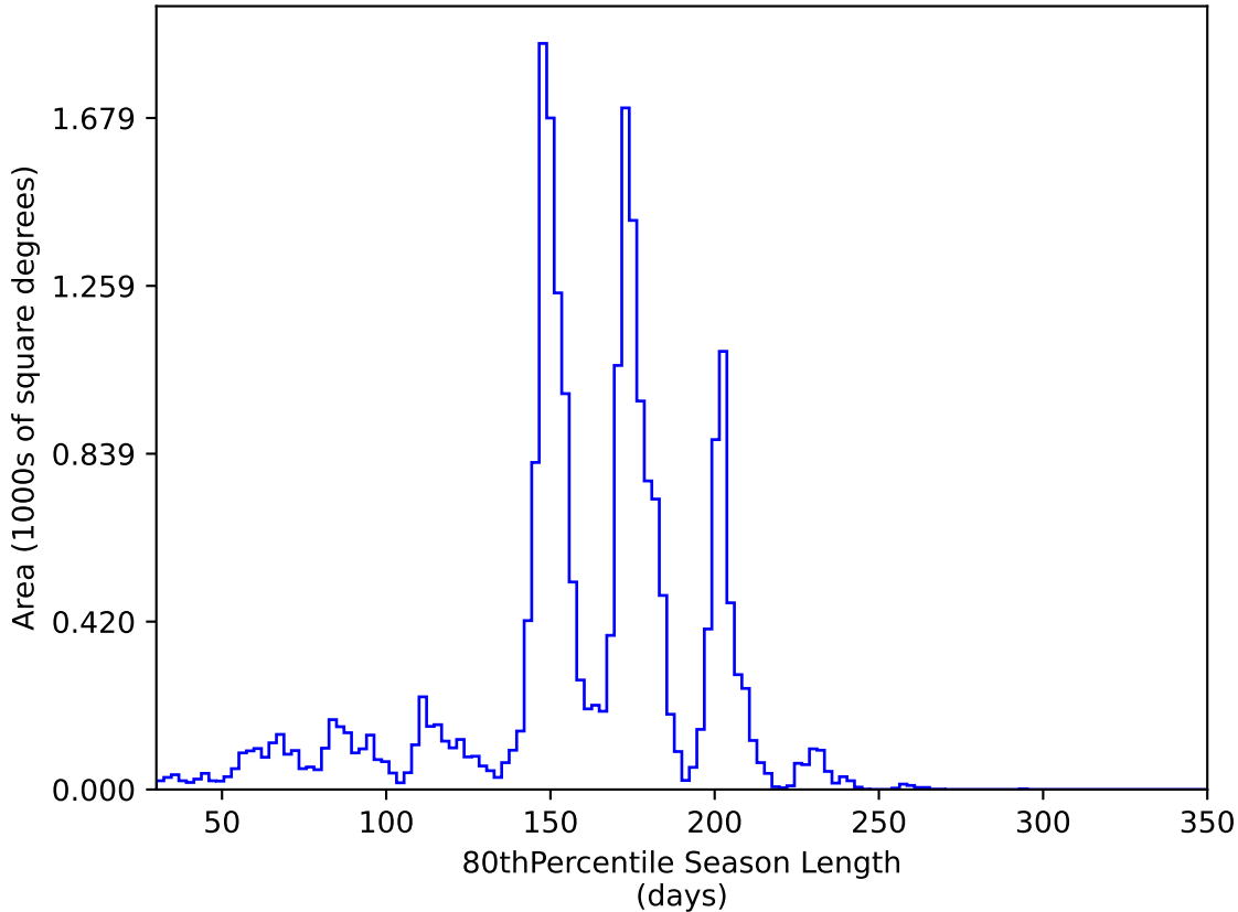
noroll_mjdp365_v3.4_10yrs All sky y band: 80thPercentile Season Length
