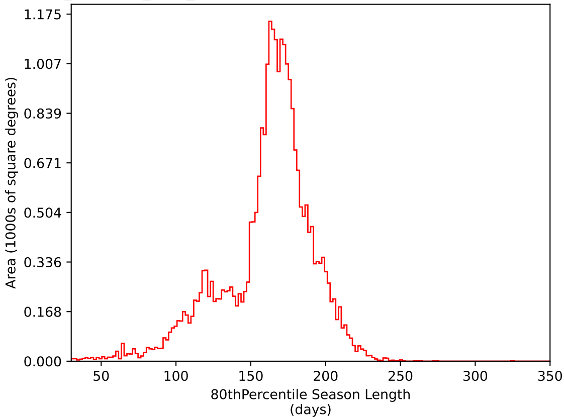
noroll_mjdp365_v3.4_10yrs All sky i band: 80thPercentile Season Length
