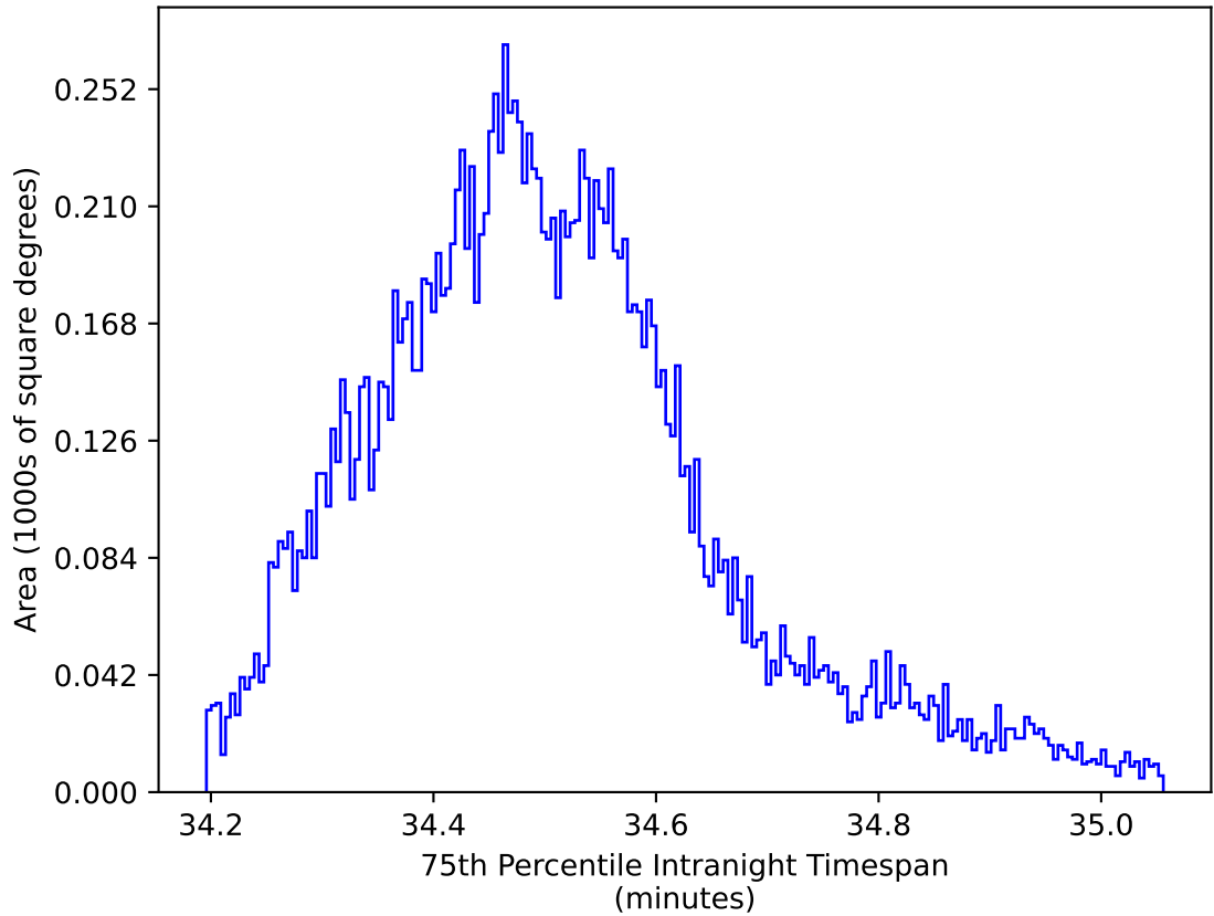
noroll_mjdp365_v3.4_10yrs WFD zy bands: 75th Percentile Intranight Timespan
