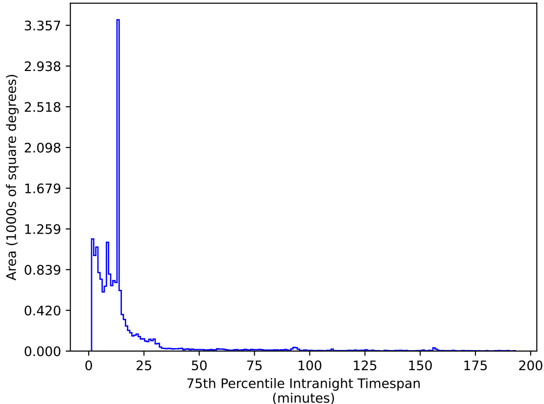
noroll_mjdp365_v3.4_10yrs WFD z band: 75th Percentile Intranight Timespan
