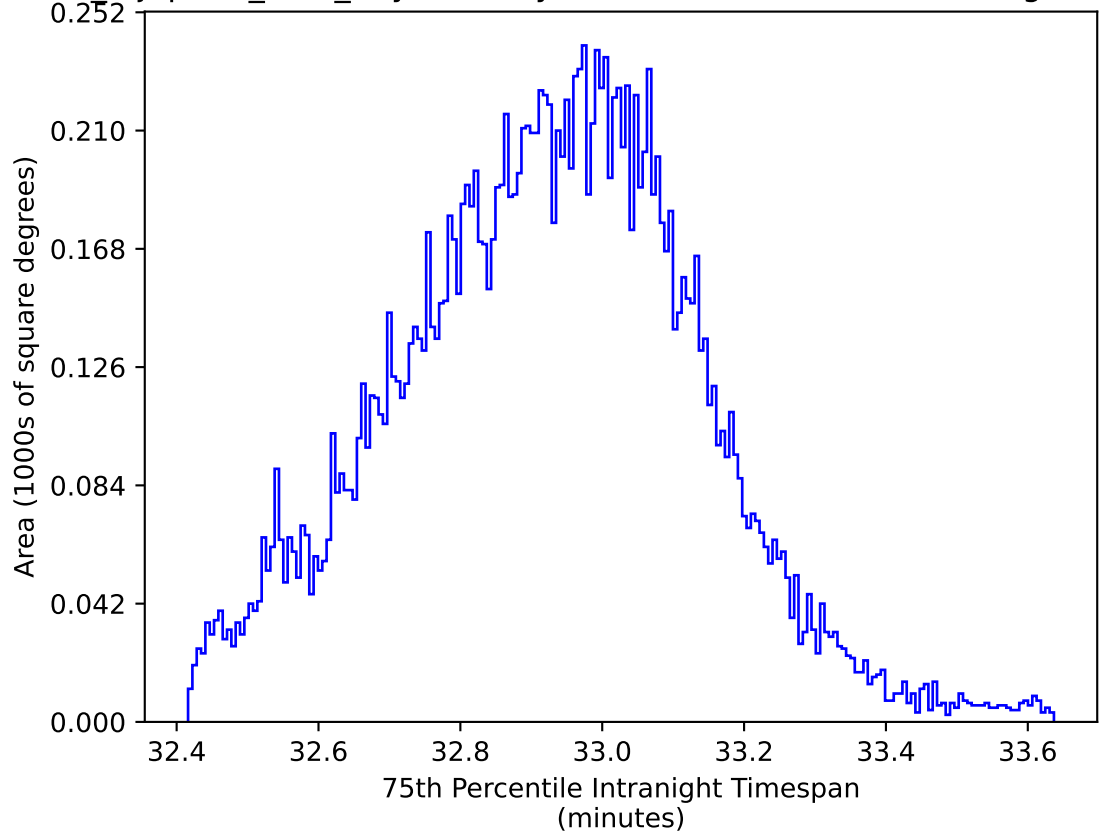
noroll_mjdp365_v3.4_10yrs WFD y band: 75th Percentile Intranight Timespan
