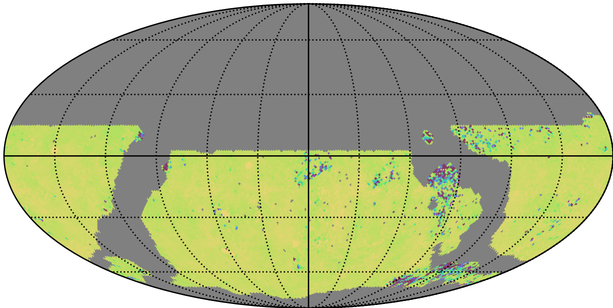
noroll_mjdp365_v3.4_10yrs WFD ug bands: 75th Percentile Intranight Timespan
