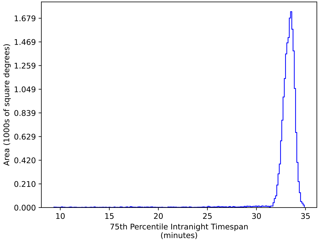
noroll_mjdp365_v3.4_10yrs WFD ug bands: 75th Percentile Intranight Timespan
