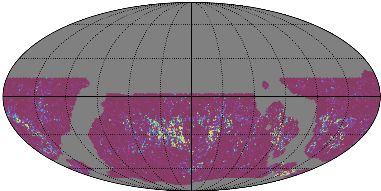
noroll_mjdp365_v3.4_10yrs WFD u band: 75th Percentile Intranight Timespan
