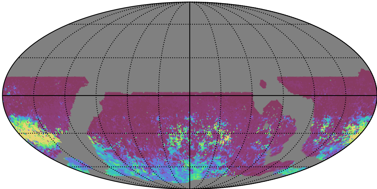
noroll_mjdp365_v3.4_10yrs WFD r band: 75th Percentile Intranight Timespan
