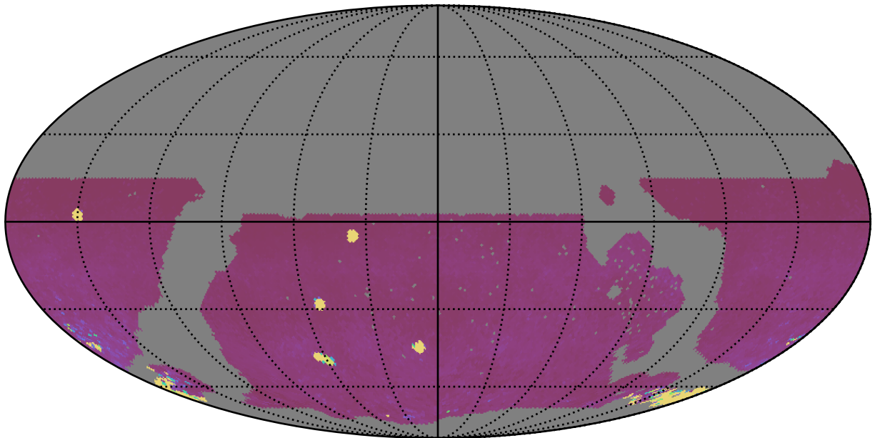
noroll_mjdp365_v3.4_10yrs WFD iz bands: 75th Percentile Intranight Timespan
