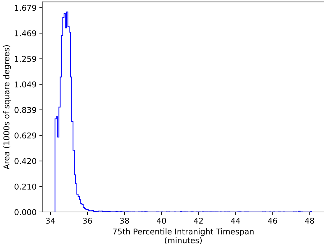
noroll_mjdp365_v3.4_10yrs WFD iz bands: 75th Percentile Intranight Timespan
