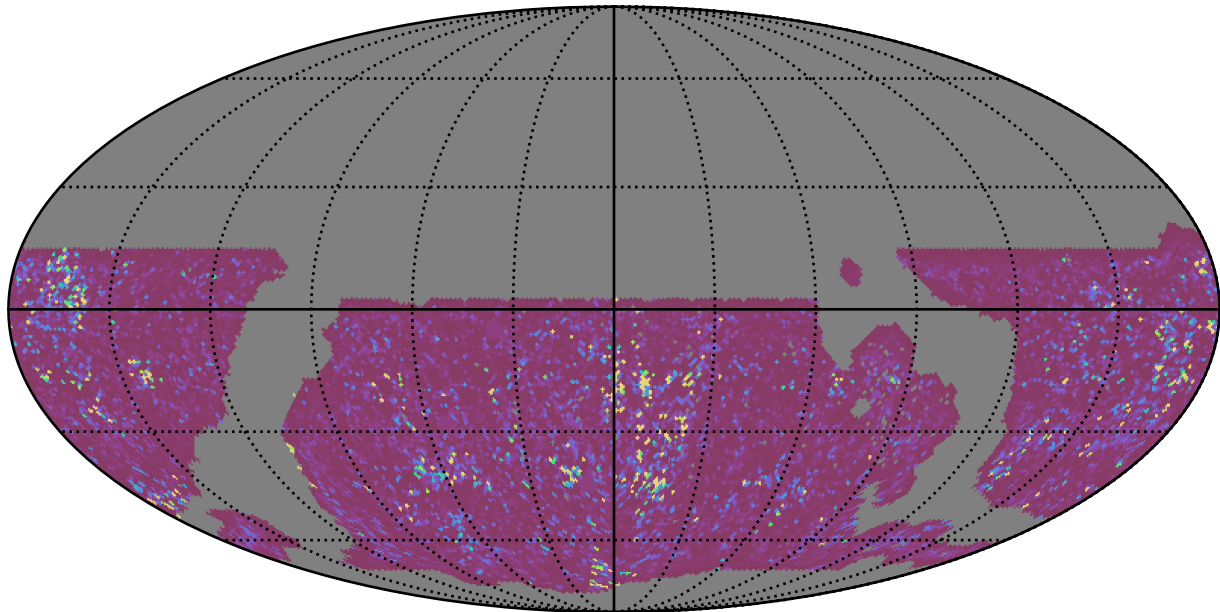
noroll_mjdp365_v3.4_10yrs WFD g band: 75th Percentile Intranight Timespan
