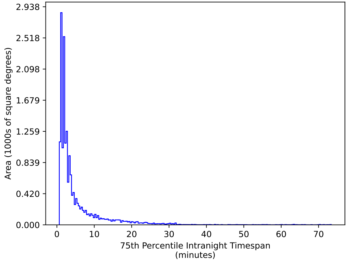
noroll_mjdp365_v3.4_10yrs WFD g band: 75th Percentile Intranight Timespan
