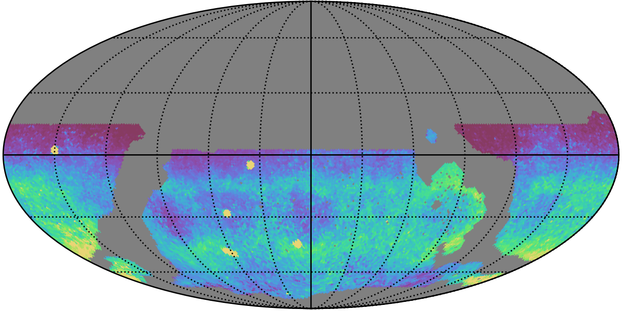
noroll_mjdp365_v3.4_10yrs WFD all bands: 75th Percentile Intranight Timespan
