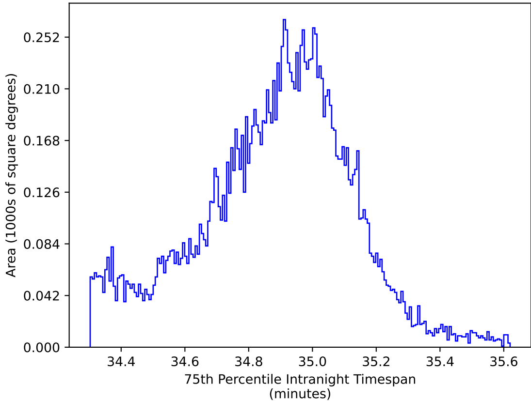
noroll_mjdp365_v3.4_10yrs WFD: 75th Percentile Intranight Timespan
