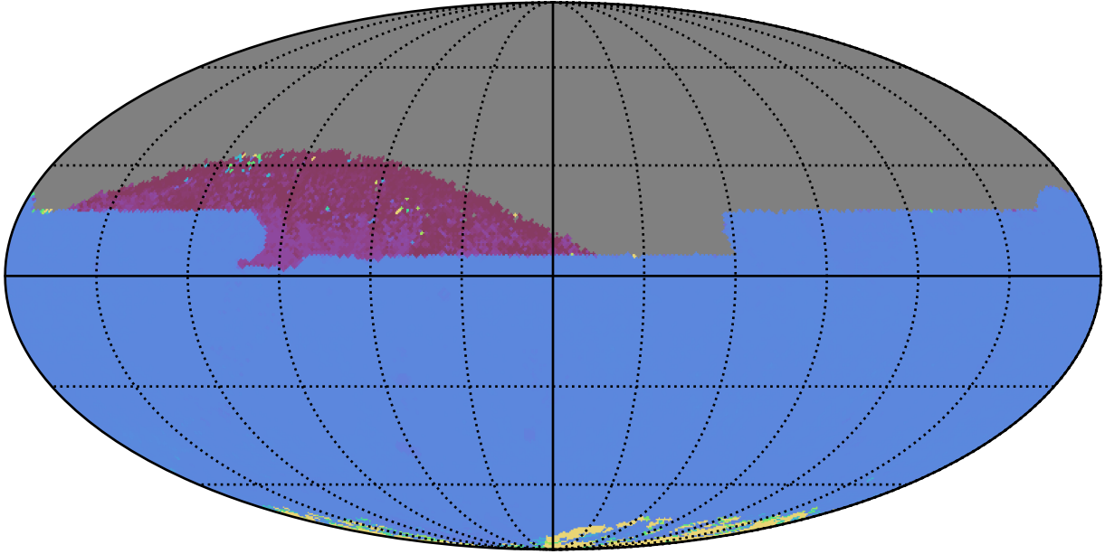
noroll_mjdp365_v3.4_10yrs All sky zy bands: 75th Percentile Intranight Timespan
