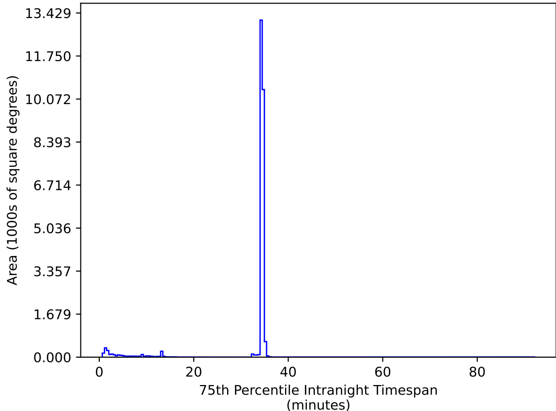
noroll_mjdp365_v3.4_10yrs All sky zy bands: 75th Percentile Intranight Timespan
