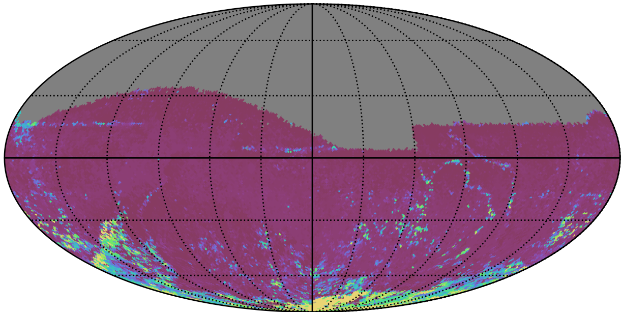
noroll_mjdp365_v3.4_10yrs All sky z band: 75th Percentile Intranight Timespan
