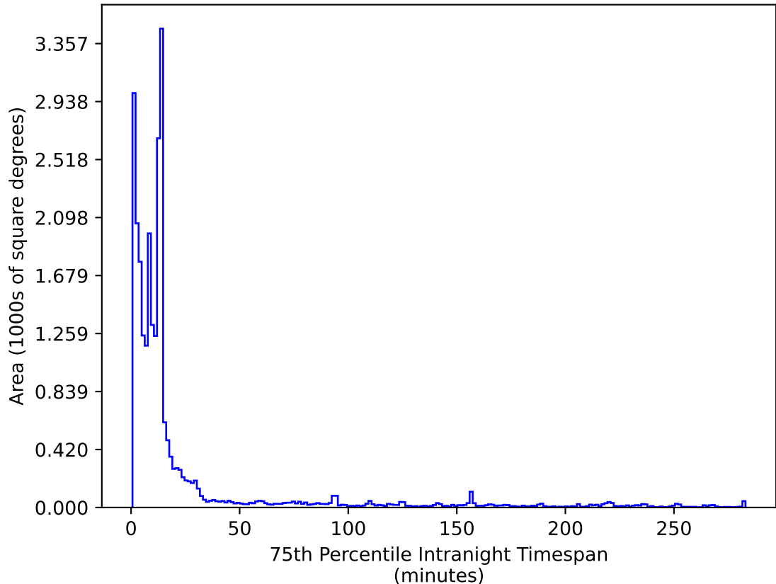
noroll_mjdp365_v3.4_10yrs All sky z band: 75th Percentile Intranight Timespan
