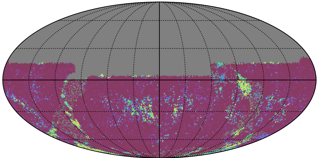
noroll_mjdp365_v3.4_10yrs All sky u band: 75th Percentile Intranight Timespan
