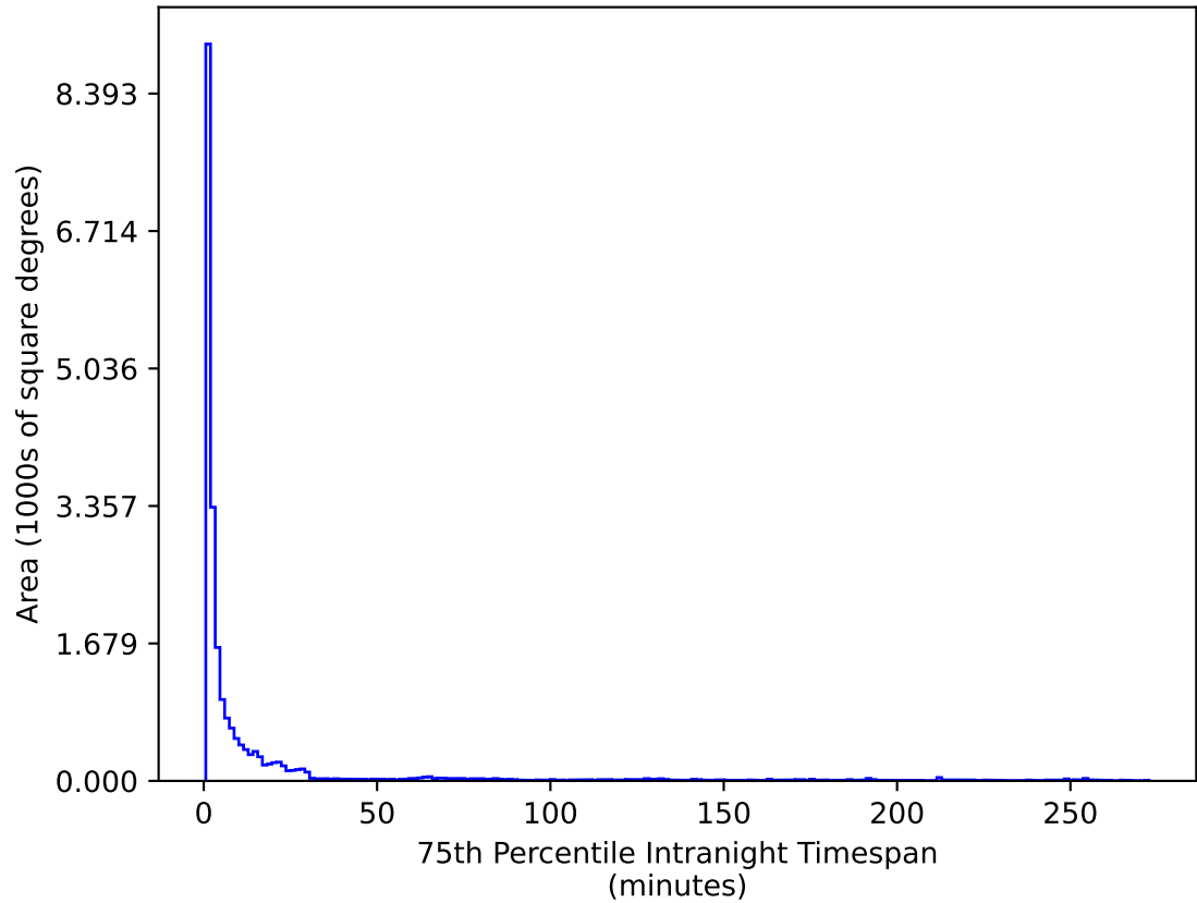
noroll_mjdp365_v3.4_10yrs All sky u band: 75th Percentile Intranight Timespan
