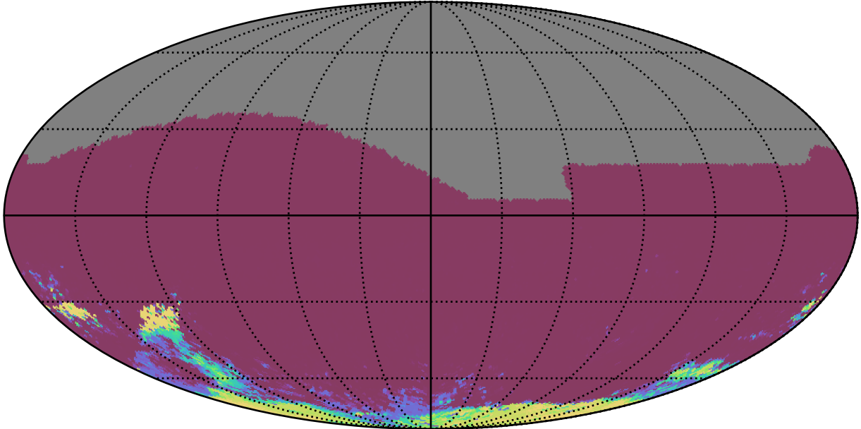
noroll_mjdp365_v3.4_10yrs All sky ri bands: 75th Percentile Intranight Timespan
