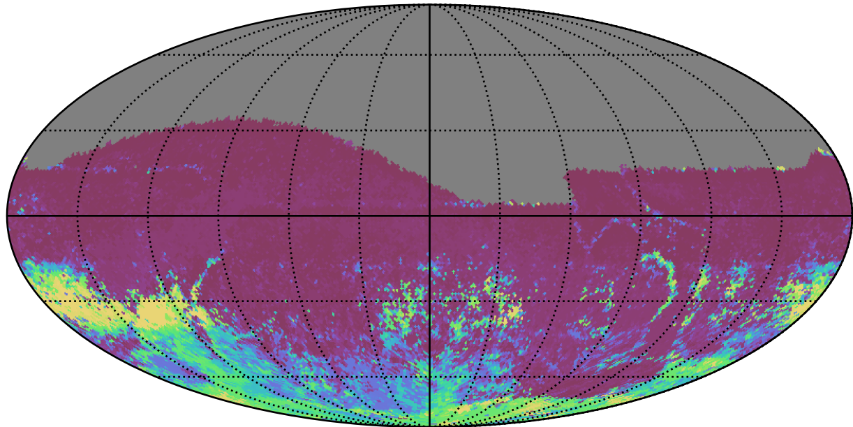
noroll_mjdp365_v3.4_10yrs All sky r band: 75th Percentile Intranight Timespan
