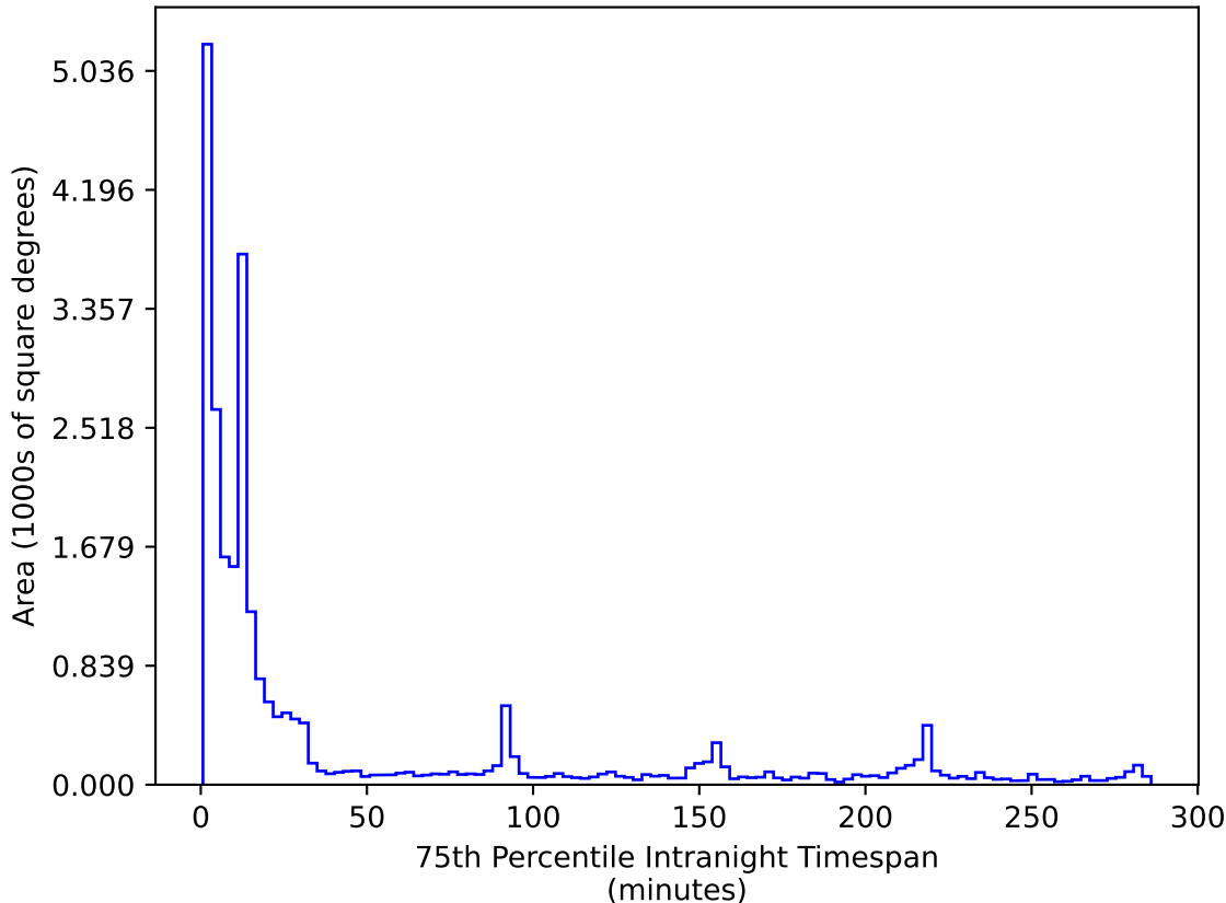
noroll_mjdp365_v3.4_10yrs All sky r band: 75th Percentile Intranight Timespan
