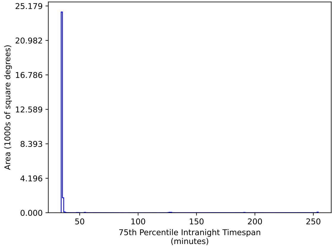
noroll_mjdp365_v3.4_10yrs All sky iz bands: 75th Percentile Intranight Timespan
