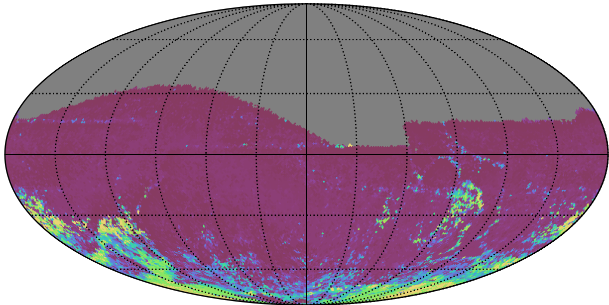
noroll_mjdp365_v3.4_10yrs All sky i band: 75th Percentile Intranight Timespan
