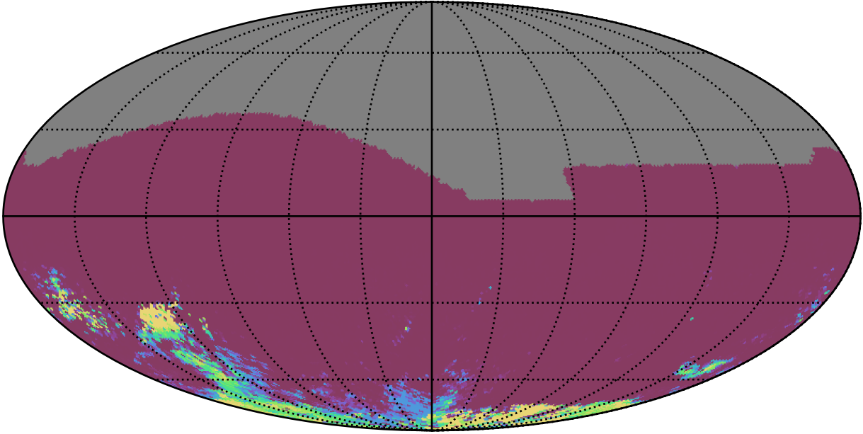
noroll_mjdp365_v3.4_10yrs All sky gr bands: 75th Percentile Intranight Timespan
