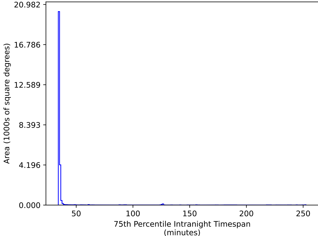
noroll_mjdp365_v3.4_10yrs All sky gr bands: 75th Percentile Intranight Timespan
